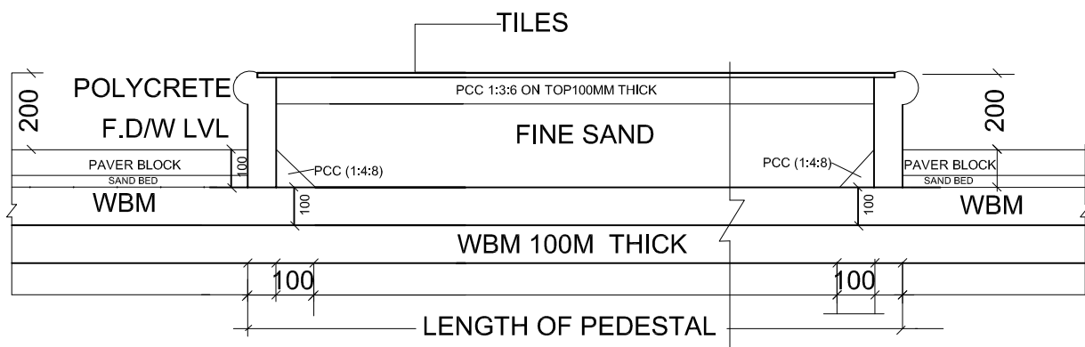
SECTION AT Y-Y
